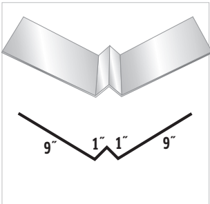
#25 Formed Valley
