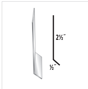
#47 Cleat
