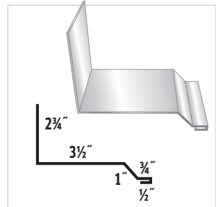
#11 Universal Sidewall
