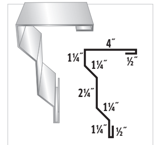
#32 Sculptured Rake
