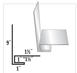
#19 Overhead Door Trim (AG) #20 Overhead Door Trim (*PBR)
