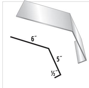
#27 Notched Gambrel
