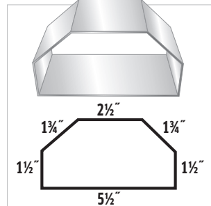
#65 Sculptured Downspout
