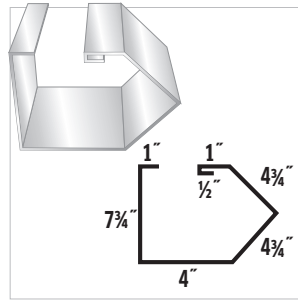
#55 Commercial Gutter
