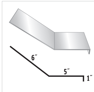
#26 Notched Endwall
