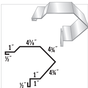
#33 Commercial Rake
