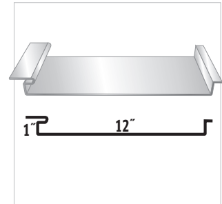
#76 Soffit Panel
