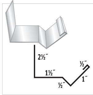
#38 Header Trim
