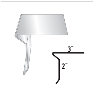
#45 Eave Trim
