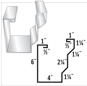
#53 Sculptured Gutter
