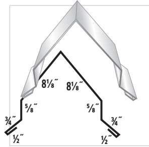
#39 XL Universal Ridge Cap
