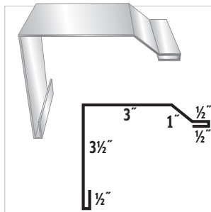
#31 Extended Rake
