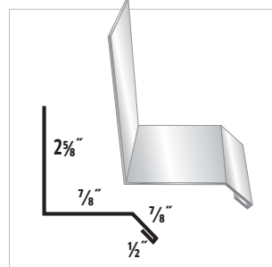
#12 Drip Cap (AG)
