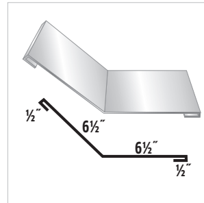
#67 Transition Flashing
