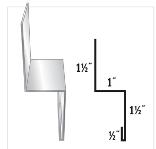
#10 Double Angle
