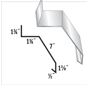
#21 Face Mount Cannon-cover
