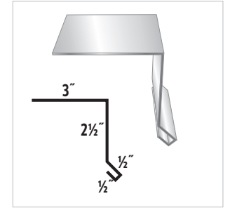
#44 Small Eave
