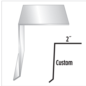
#43 Rake Cleat
