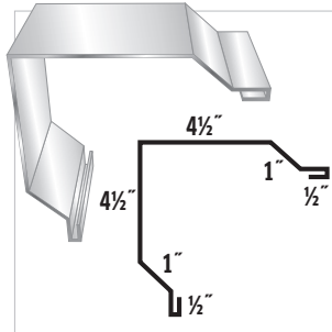
#3 Rake & Corner
