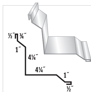
#18 Inside Corner
