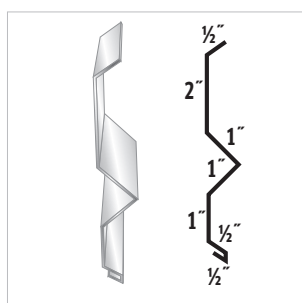
#34 Headwall Counter Flashing
