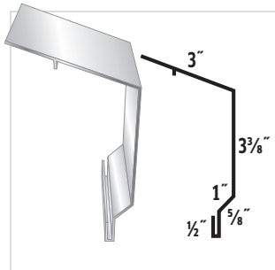
#6 Fascia Trim
