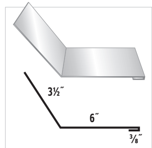
#15 Universal Endwall
