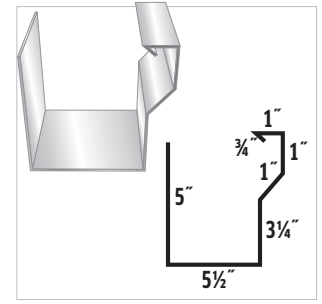
#56 Gutter
