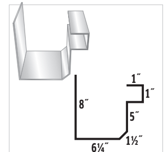
#52 Commercial Gutter
