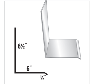
#28 "L" Flashing
