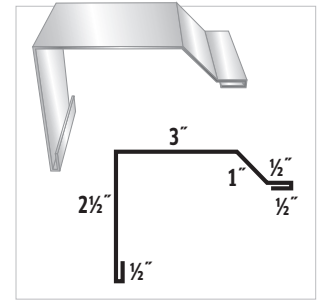
#24 Residential Rake
