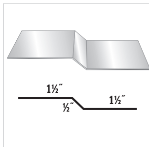
#30 Offset Cleat
