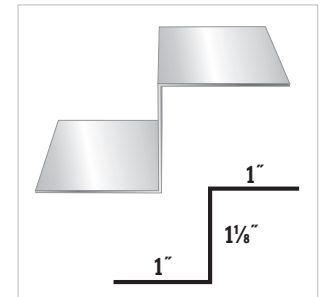
#48 Z Flashing
