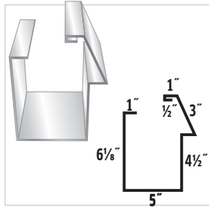
#54 Commercial Gutter
