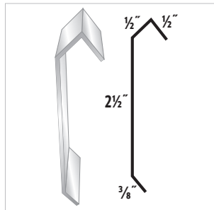
#46 "F" Slip Track
