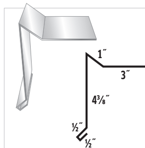
#35 Gravel Stop
