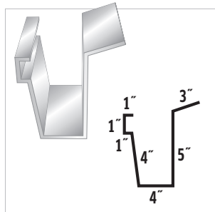
#50 Eave Gutter - Small
