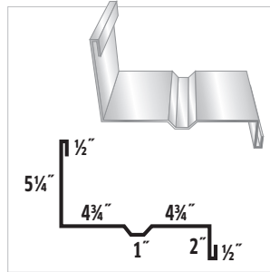
#23 One Piece Fascia & Soffit
