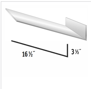
#81 Chimney Flashing
