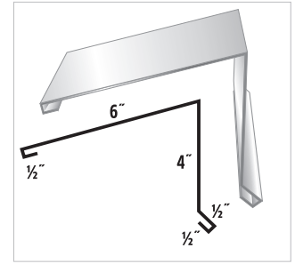
#80 Peak Cap
