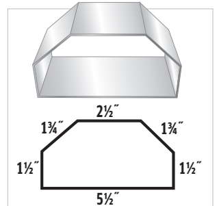
#65 Sculptured Downspout
