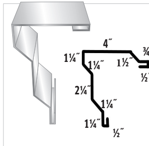
#32 Sculptured Rake
