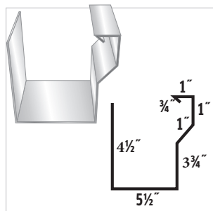
#56 Gutter
